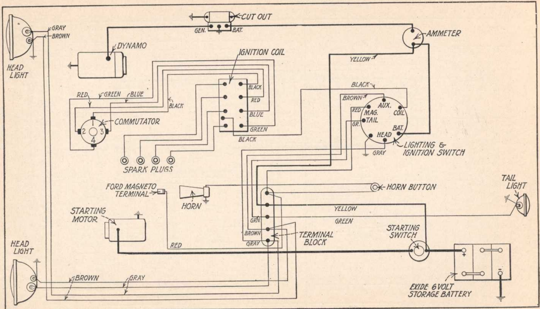
Fig. 87. Wiring Diagram with Cutout on Dash
