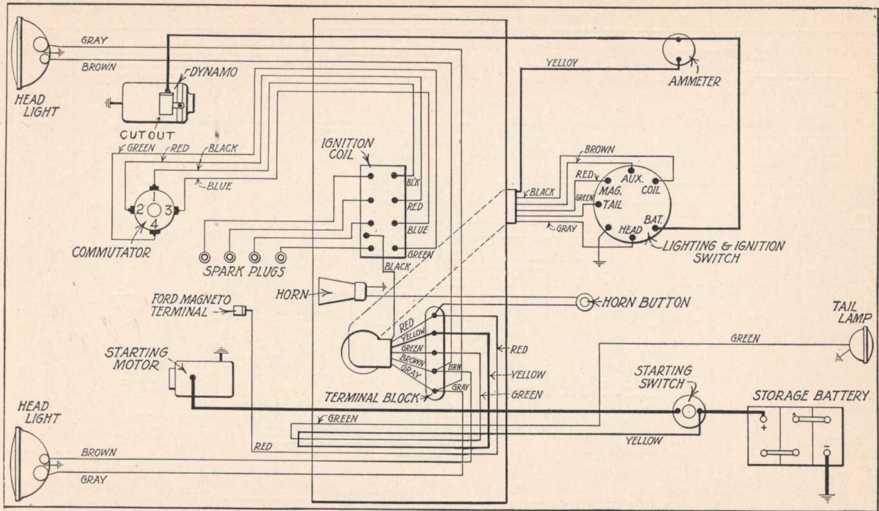
Fig. 88. Wiring Diagram with Cutout on Generator
